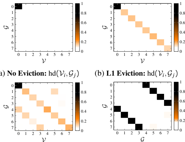
(a) No Eviction: hd(\mathcal{V}_i, \mathcal{G}_j) (b) L1 Eviction: hd(\mathcal{V}_i, \mathcal{G}_j) (c) L1+L2 Eviction: hd(\mathcal{V}_i, \mathcal{G}_j) (d) L1+L2 Eviction: hd(\mathcal{G}_i, \mathcal{G}_j) Figure 4: Coefficients for the sliced components hd(\mathcal{V}_i, \mathcal{G}_j) for all eviction techniques and hd(\mathcal{G}_i, \mathcal{G}_j) for L1+L2 eviction. We see that the structure of the power model changes based on the eviction technique and additional unaligned effects.
